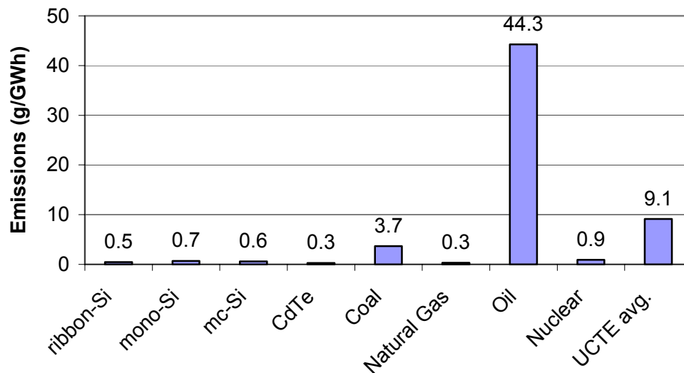
Figure 1. Life-cycle atmospheric Cd emissions for PV systems normalized for Southern Europe’s average insolation of 1700 kWh/m 2 /yr, performance ratio of 80%, and lifetime of 30 yrs. Each PV system is assumed to include a ground-mount BOS as described by Mason et al. [11].
