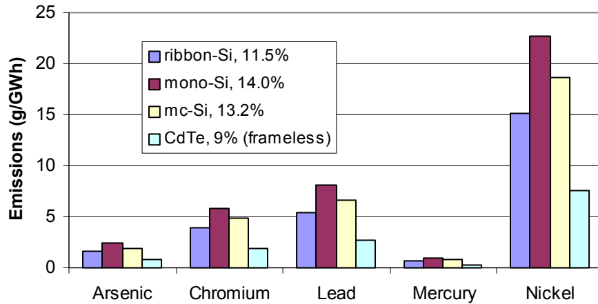
Figure 2. Emissions of heavy metals due to electricity use, based on European UTCE averages (Ecoinvent database)
